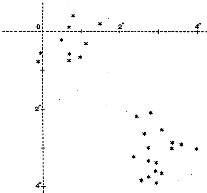
FIG. 4.—Moving Cluster of "Orion" Stars in Perseus.
